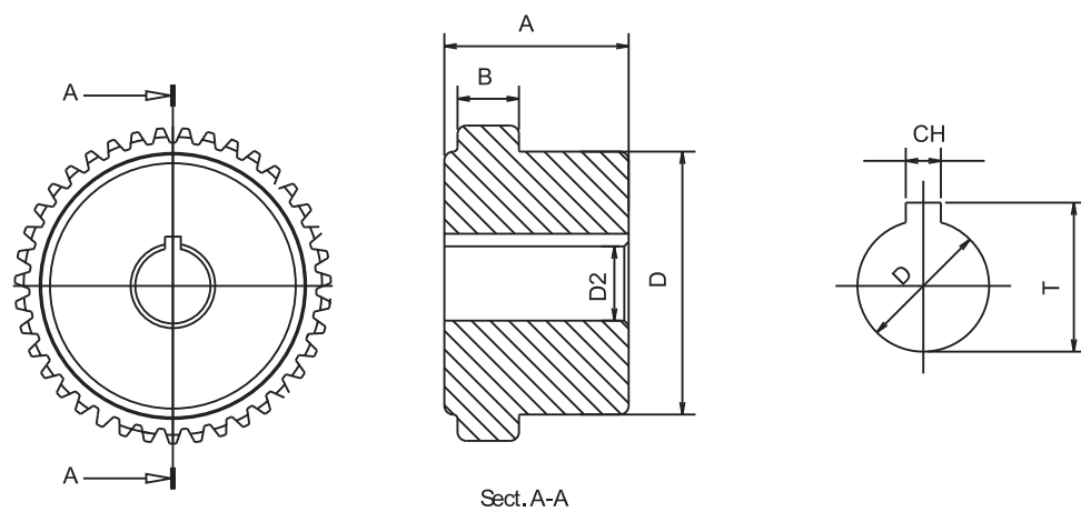
Sect. A-A
